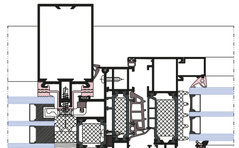
Facade and window connection
